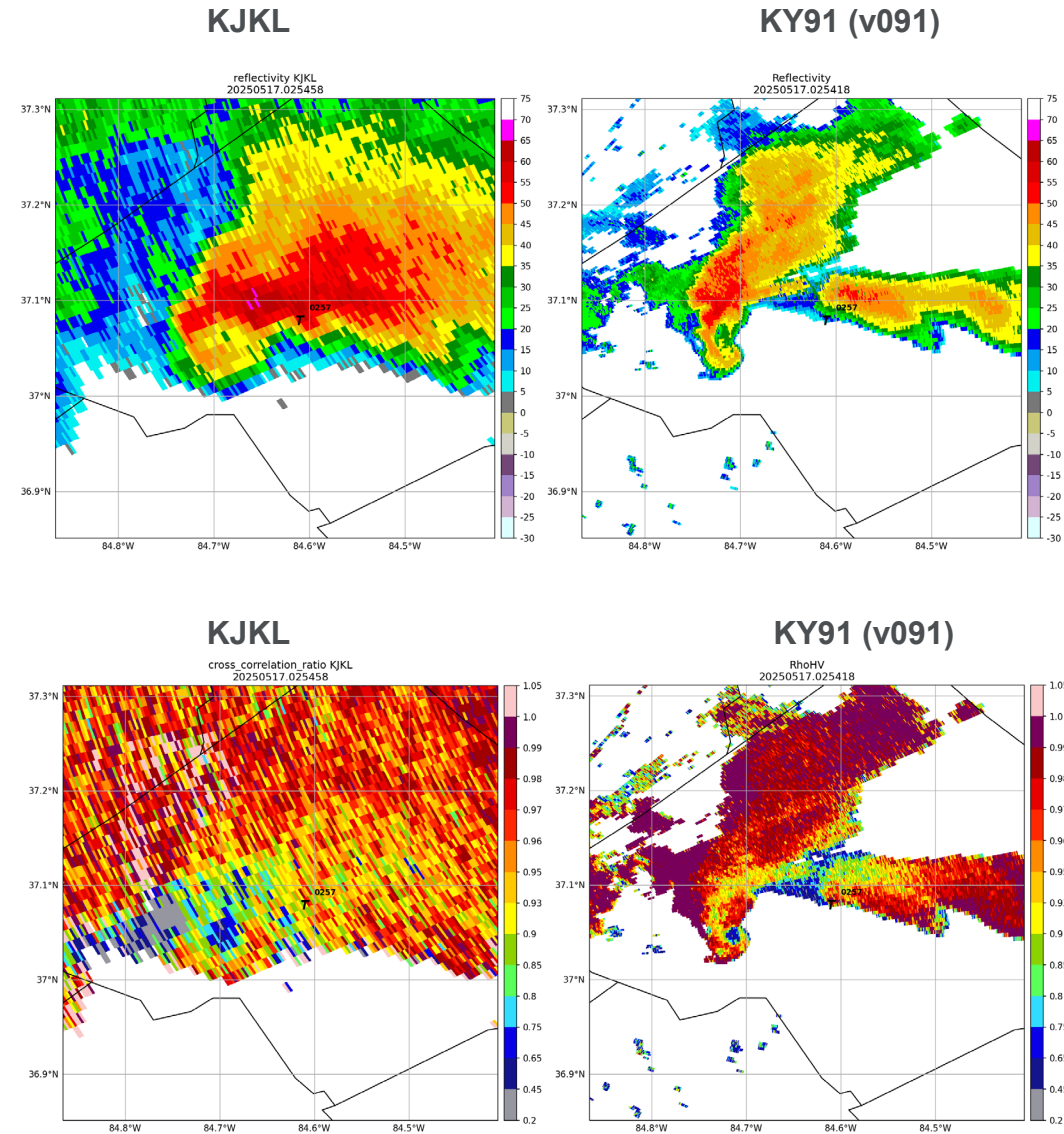
Reflectivity (top) and RhoHV (bottom) data from Climavision's KY91 (v091) radar and KJKL.
